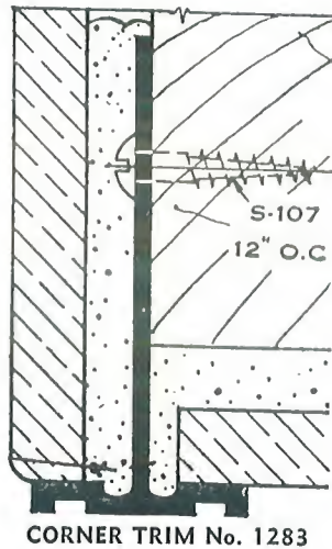
EXTRUDED MOULDINGS FOR STRUCTURAL GLASS (ALUMINUM AND BRONZE)
